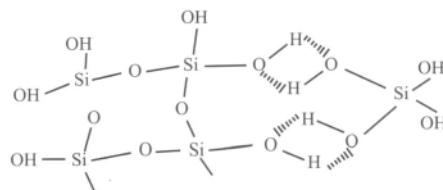
图1 KH560与TEOS形成的网络结构示意图 Fig.1 The network structure schematic drawing of the combination of KH560 and TEOS
