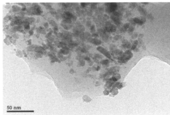
图2 有机硅处理剂的透射电子显微镜照片 Fig.2 TEM images of organic silicon treatment
